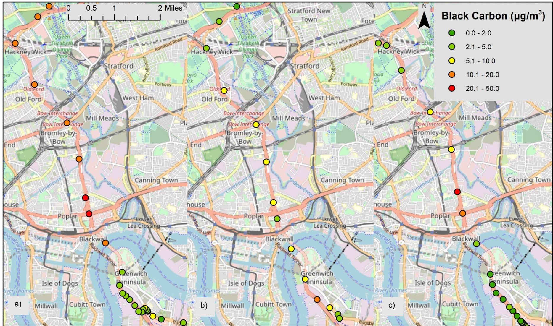
Figure 7: High BC exposure events travelling through the Blackwall Tunnel by a heavy freight driver (DEM013). a) South to north at 08:00 on 14 February 2018; b) North to south at 09:00 on 14 February 2018; c) South to north at 09:00 on 15 February 2018. Each dot represents one-minute of exposure.
